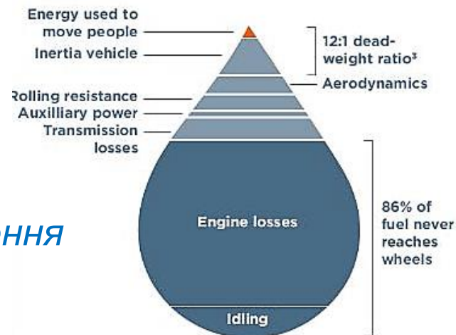
TANK-TO-WHEEL ENERGY FLOW - PETROL
